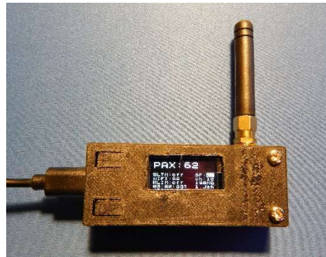
Fig.5 LoRa module (author's photo)
